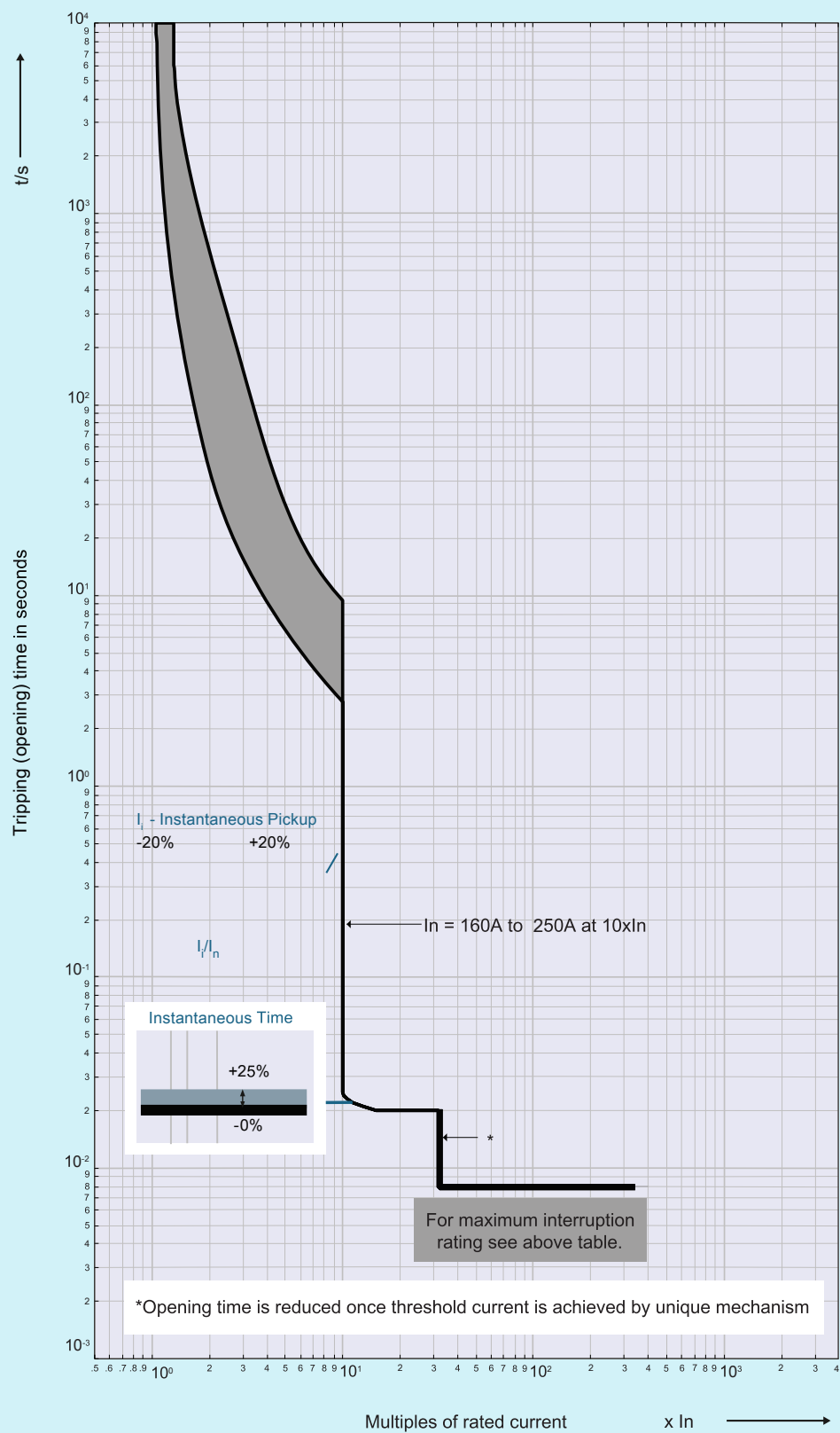
3VJ12 160A-250A FTFM trip unit
