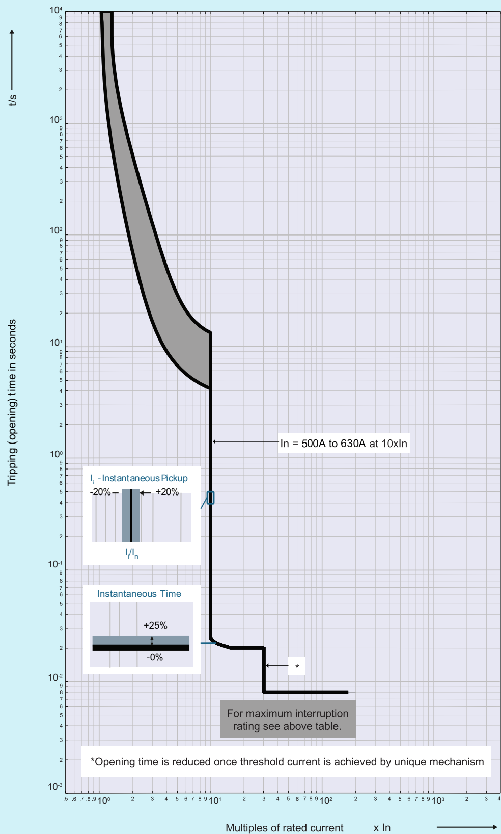
3VJ13 320A-400A ATFM trip unit
