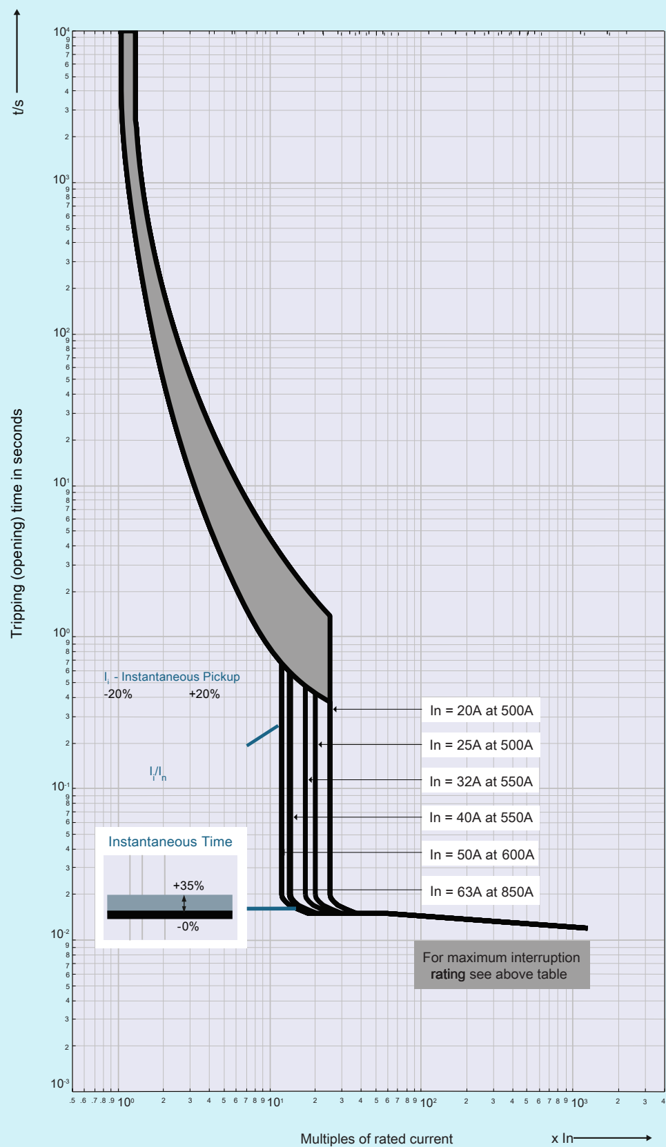
3VJ10 20A-63A ATFM trip unit
