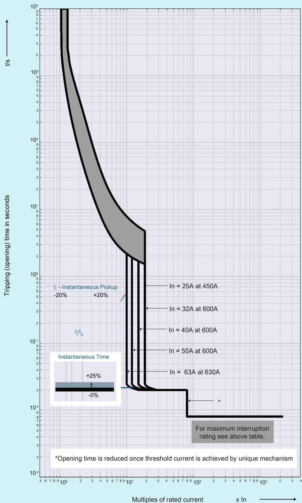
3VJ11 25A-63A ATFM trip unit
