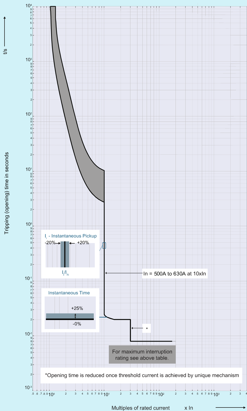
3VJ14 500A-630A FTFM trip unit
