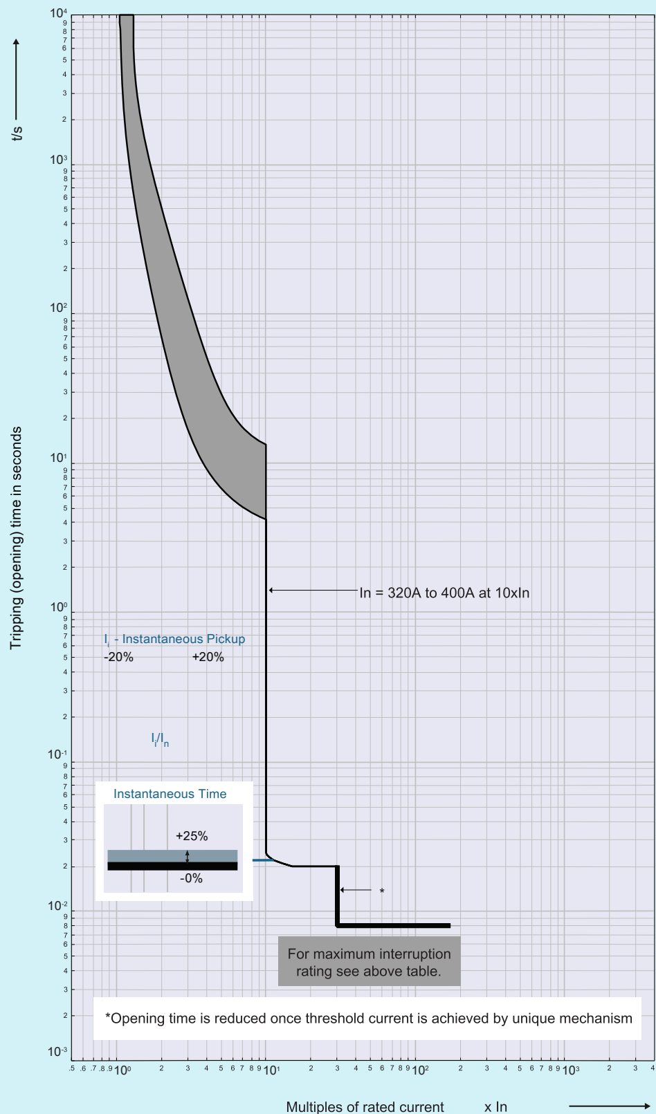
3VJ13 320A-400A FTFM trip unit
