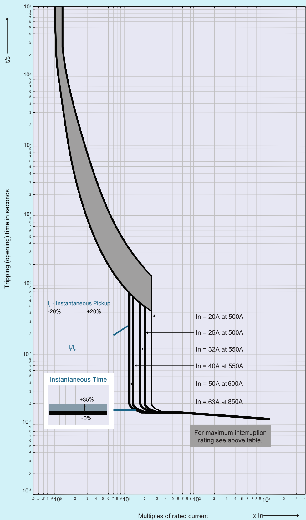
3VJ10 20A-63A FTFM trip unit
