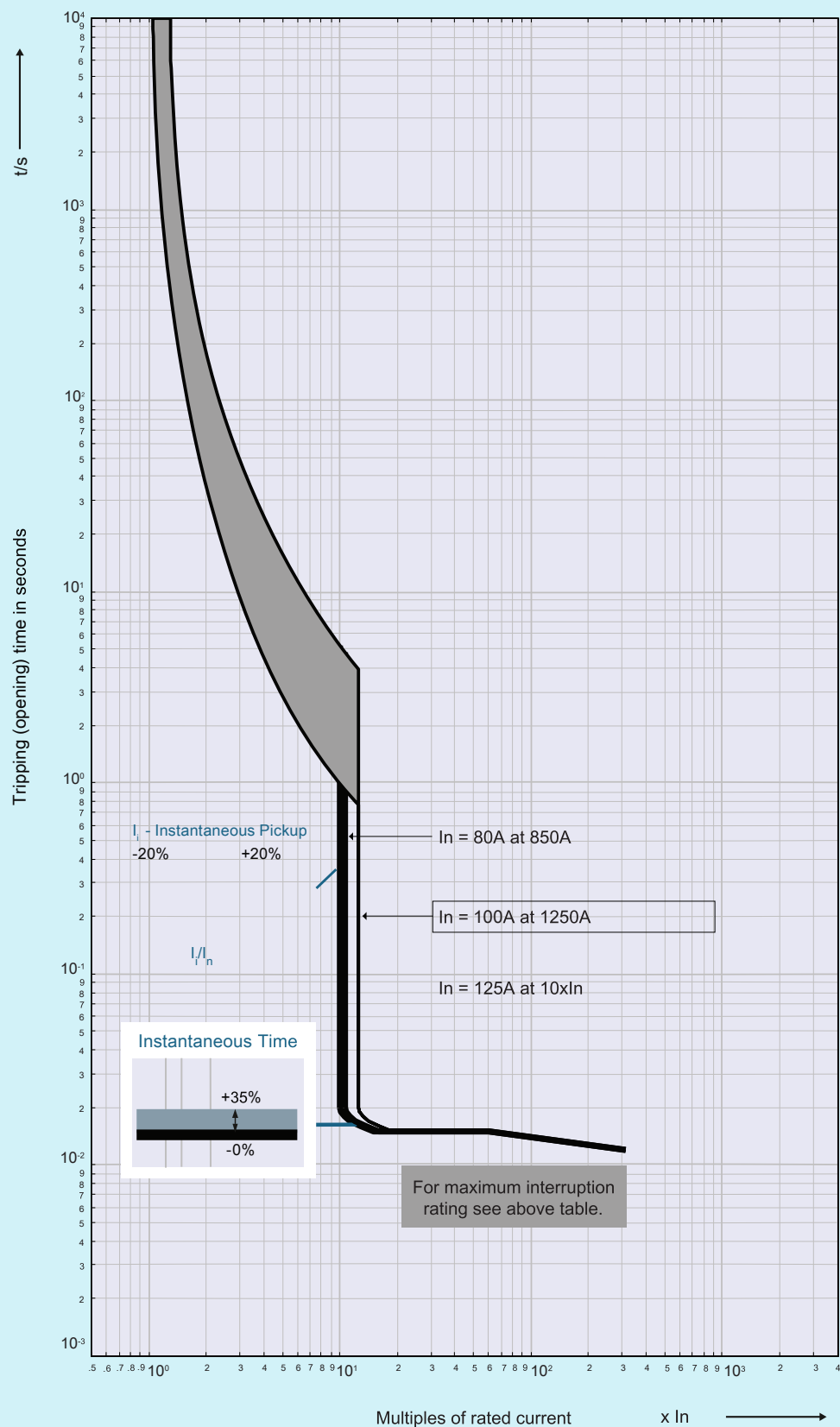
3VJ10 80A-125A FTFM trip unit
