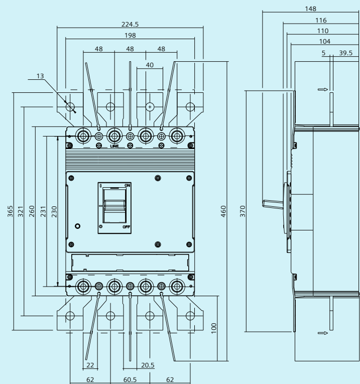
Frame 3 | 3VJ13 4P
