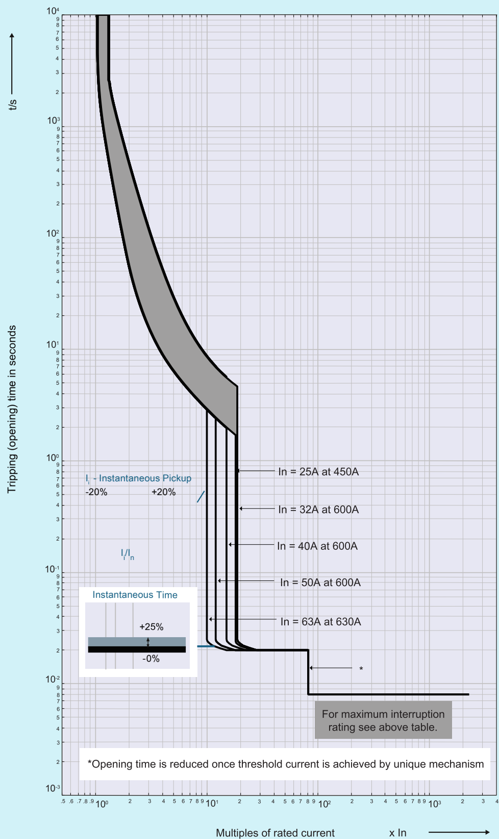
3VJ11 25A-63A FTFM trip unit
